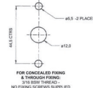
FIXING HOLE DETAILS
