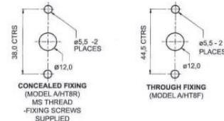
FIXING HOLE DETAILS
